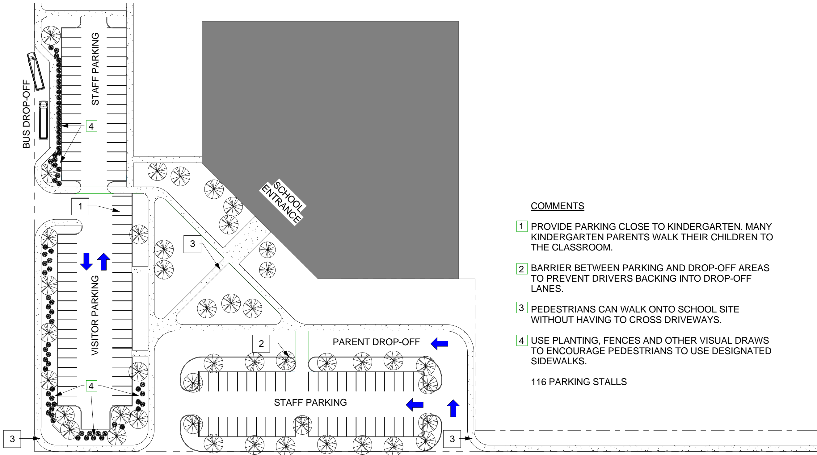
1 Site Plan 1" = 50'-0"
